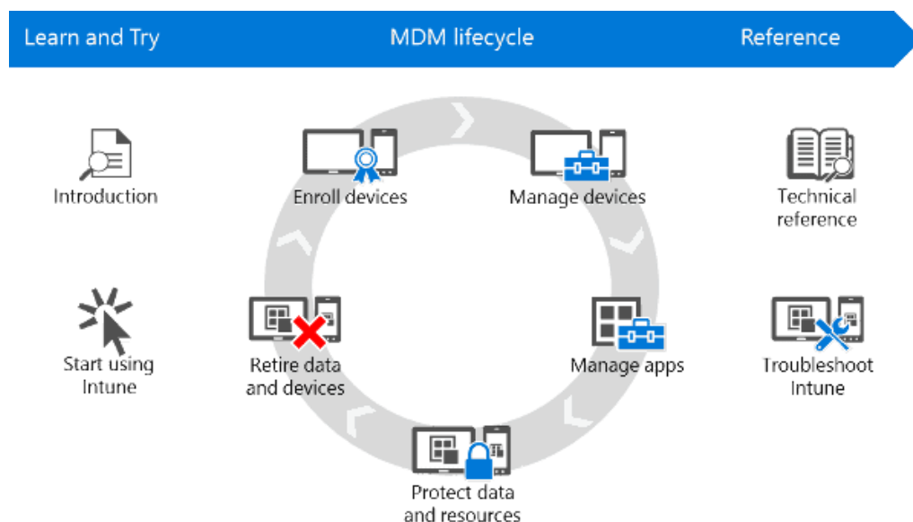
Figure 2: Intune lifecycle 38
